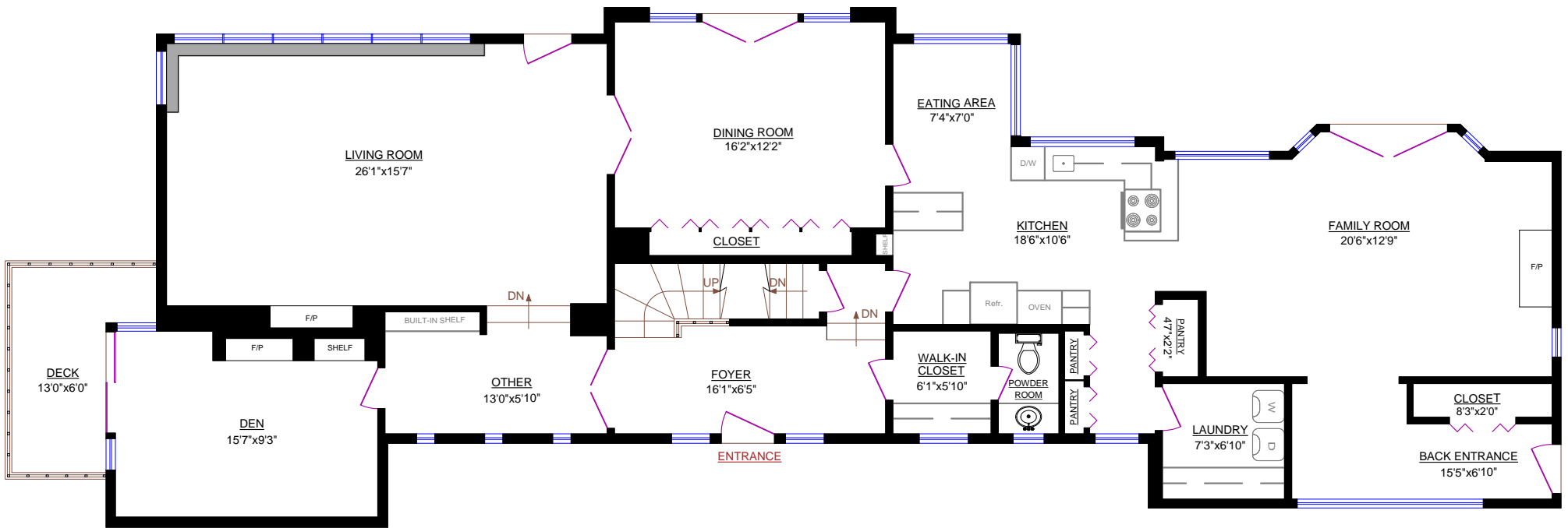
MAIN FLOOR
